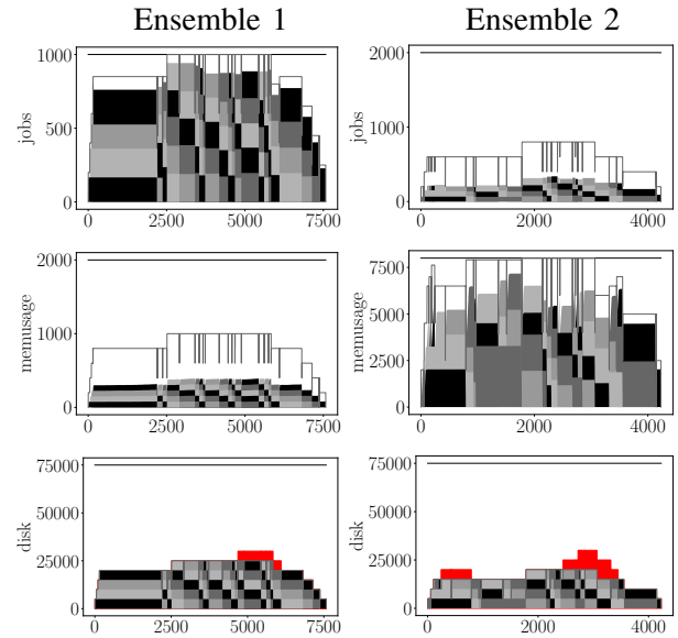
Fig. 2: Workflow Resource Control
